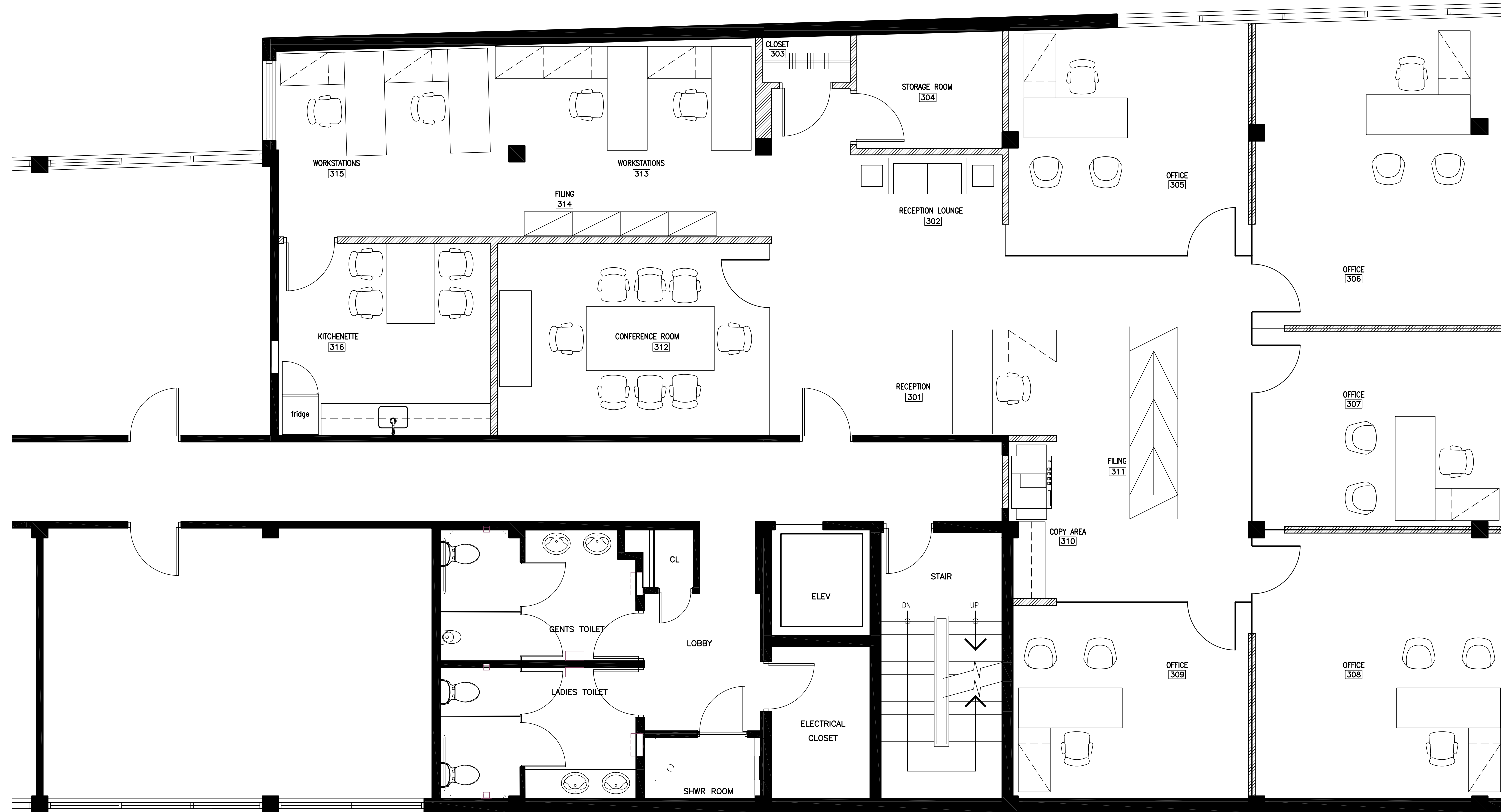
1 FURNITURE PLAN 3-03 SCALE: 1/4"=1'-0"
